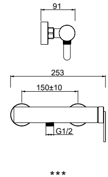
16912000072 (Ø35) Shower Mixer
