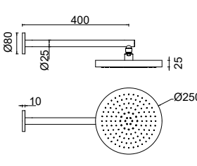
SH908372-2 Rain Shower Head 10"
