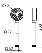
HS913572 Hand Shower
