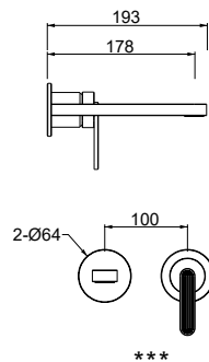
16913360072 (Ø35) Wall Mounted Basin Mixer
