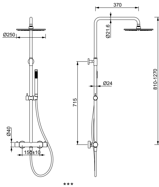
16208140072 Thermostatic Rain Shower Set
