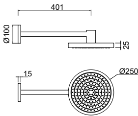
SH908372 Rain Shower Head 10"
