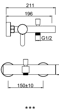
16911000072 (Ø35) Bath Shower Mixer
