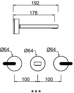
16913180072 (G1/2) Wall Mounted Basin Mixer
