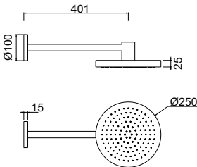
SH908372-1 Rain Shower Head 10"
