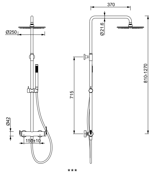
169181000 (Ø35) Rain Shower Set
