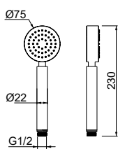
HS913572-1 Hand Shower
