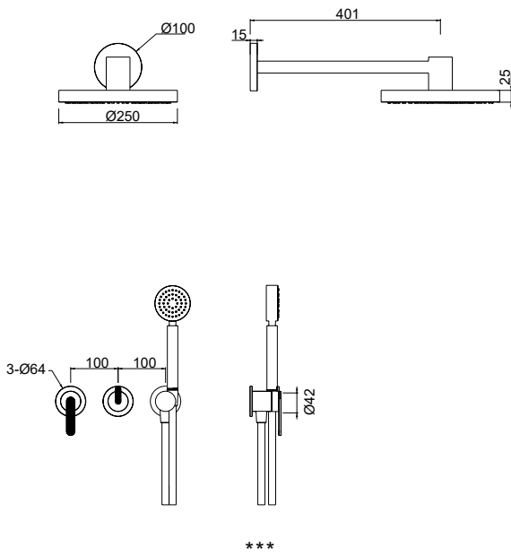
16911740072 (Ø35) (2-Function) Concealed Rain Shower Set
